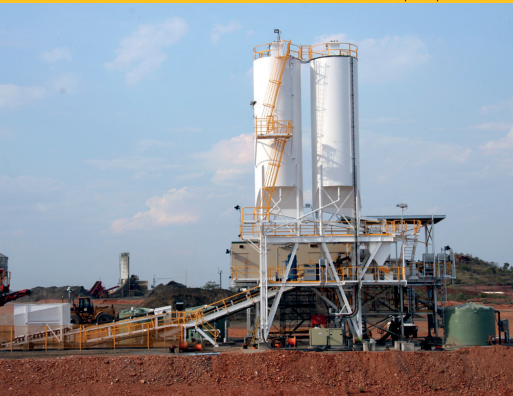
Static backfill paste plant
